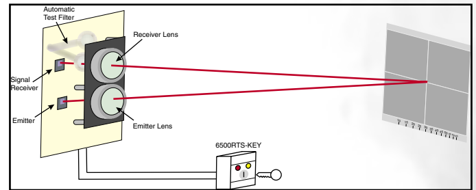
Figure 9: 6500 Beam Detector Asuretest Operation
