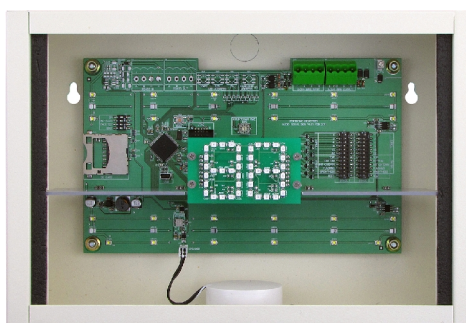
Audio-Visual Sign (AVS-C) with Fascia removed
