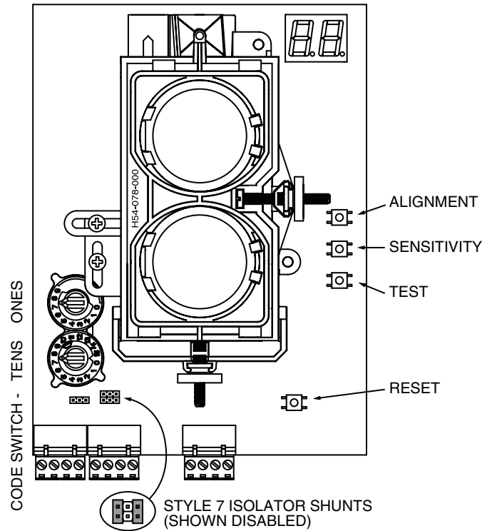
FIGURE 10. SWITCH LOCATIONS:
