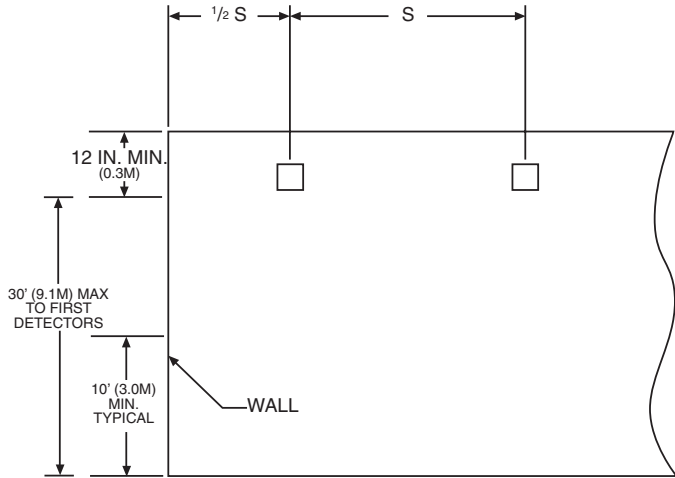
FIGURE 1. SPACING FOR SMOOTH CEILING (SIDE VIEW):
