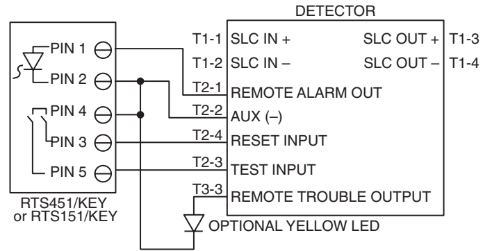
FIGURE 8. WIRING DIAGRAM (RTS451 OR RTS151):
