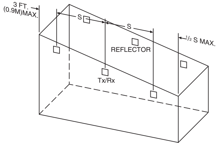
FIGURE 3. SLOPED CEILING (SHED TYPE):
