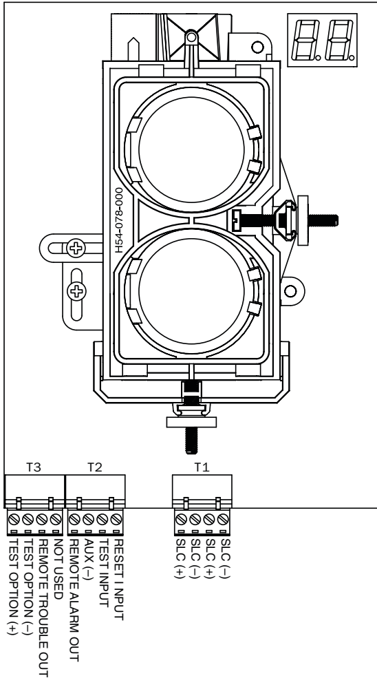
FIGURE 7. WIRING DIAGRAM:
