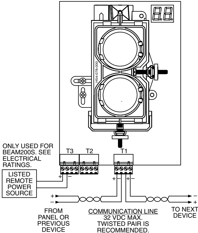
FIGURE 7. WIRING DIAGRAM:
