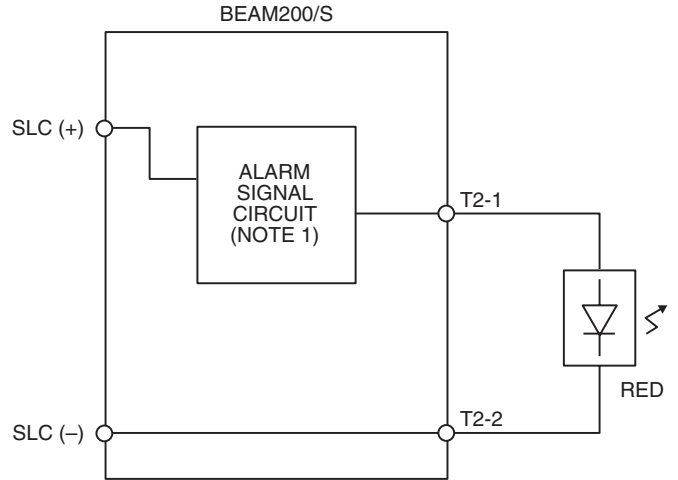
FIGURE 9. WIRING DIAGRAM (RTS451 OR RTS151):
