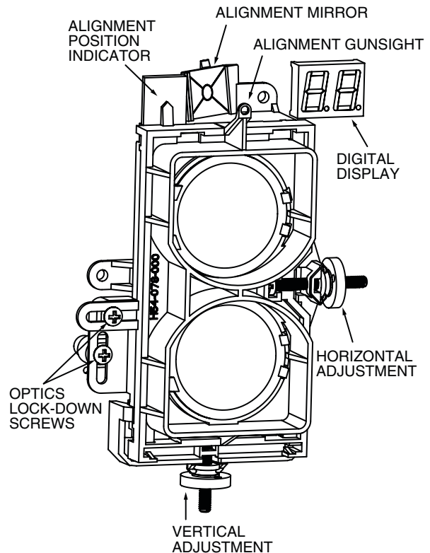
FIGURE 11. ALIGNMENT ADJUSTMENT LOCATIONS:
