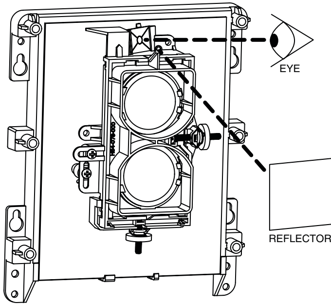
FIGURE 12. COARSE ALIGNMENT PROCEDURE:
